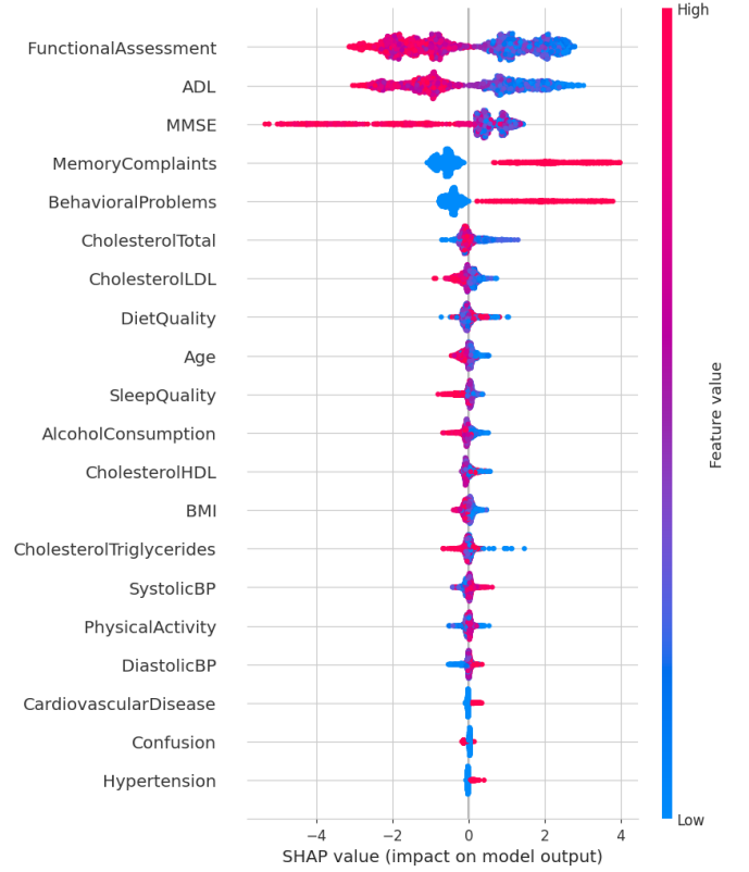
Fig. 9. SHAP summary (LightGBM, Full track). Assessment features dominate the model output; screening features cluster at zero.
